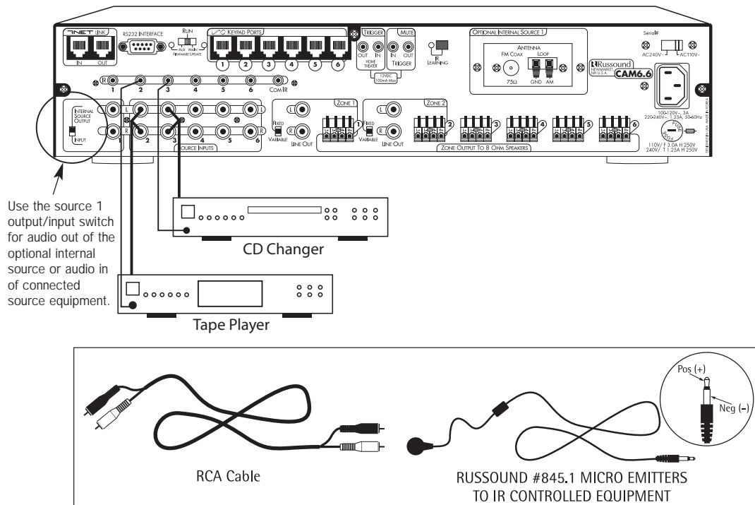
CAM6.6 with Optional Internal Source - AM/FM Tuner
